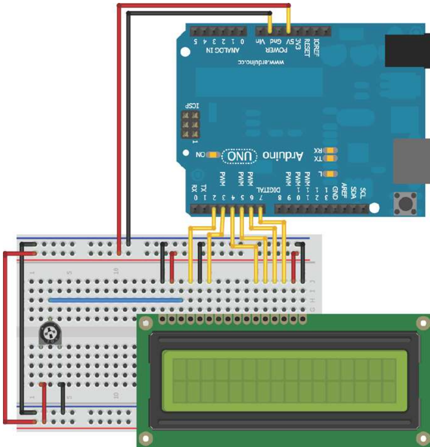
Figure 10-2: LCD wired to breadboard and Arduino
