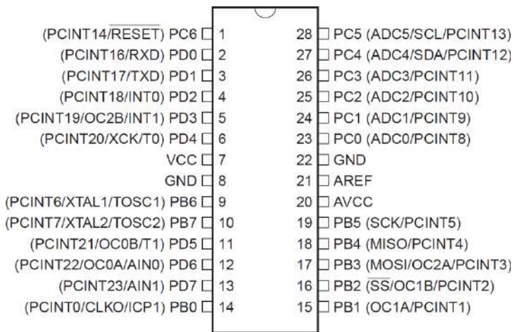
Figure A-3: ATmega 328p DIP pin-out
