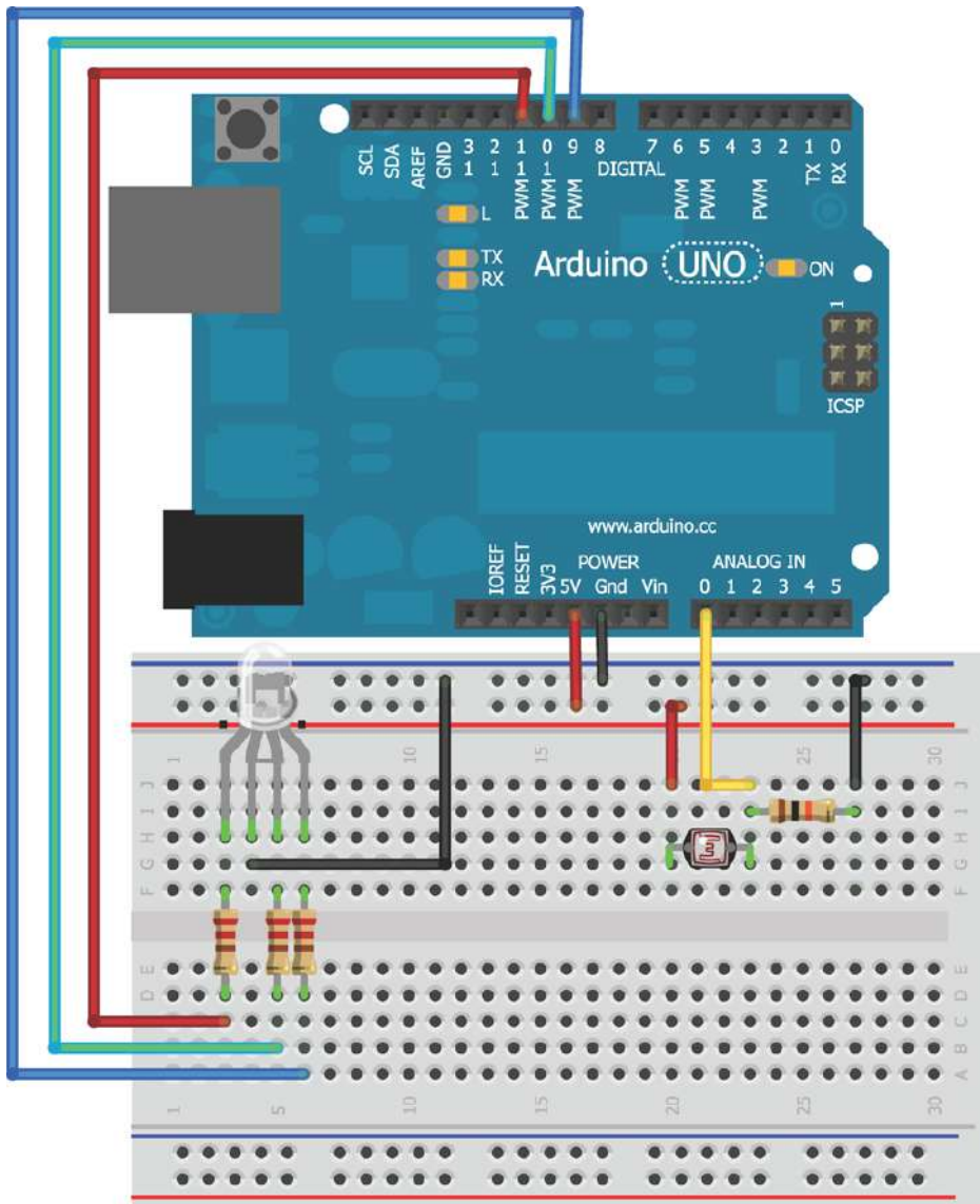
Figure 3-11: Photoresistor circuit
