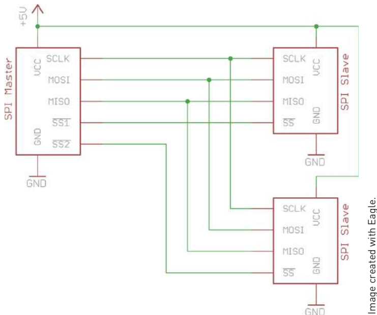
Figure 9-1: SPI reference hardware configuration
