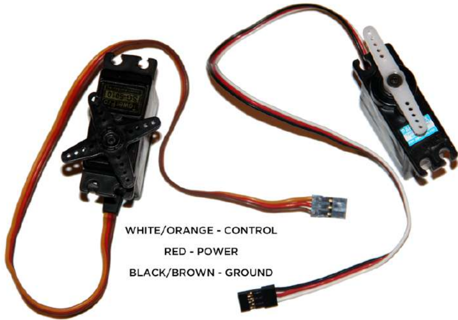
Figure 4-9: Servo motors
