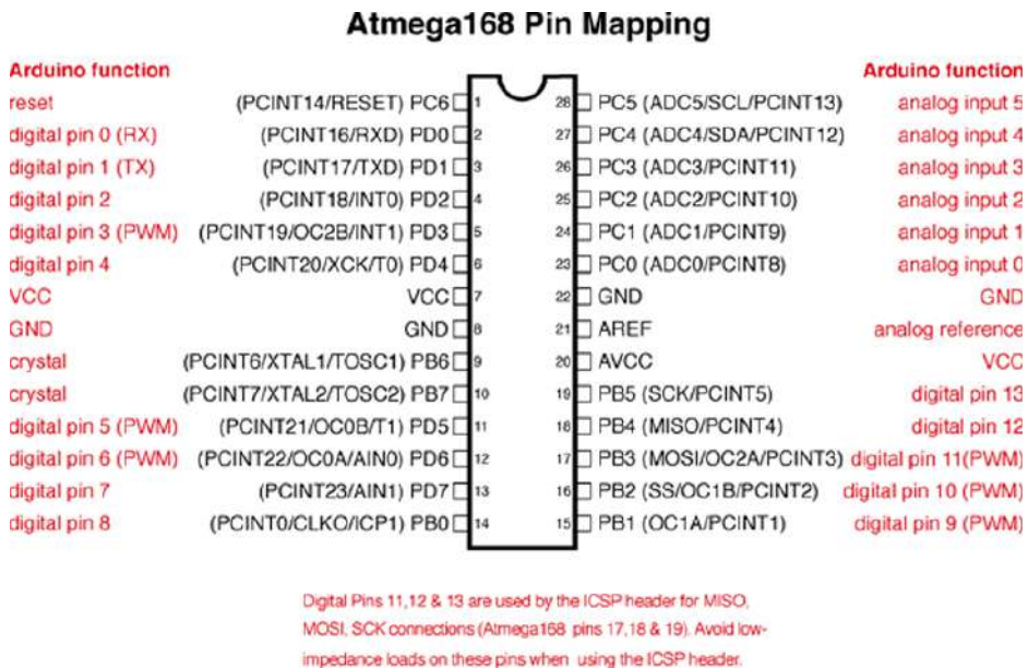
Figure A-4: Arduino ATmega Pin Mapping
