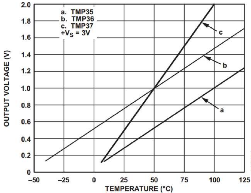
Figure 3-7: Voltage to Temperature Correlation
