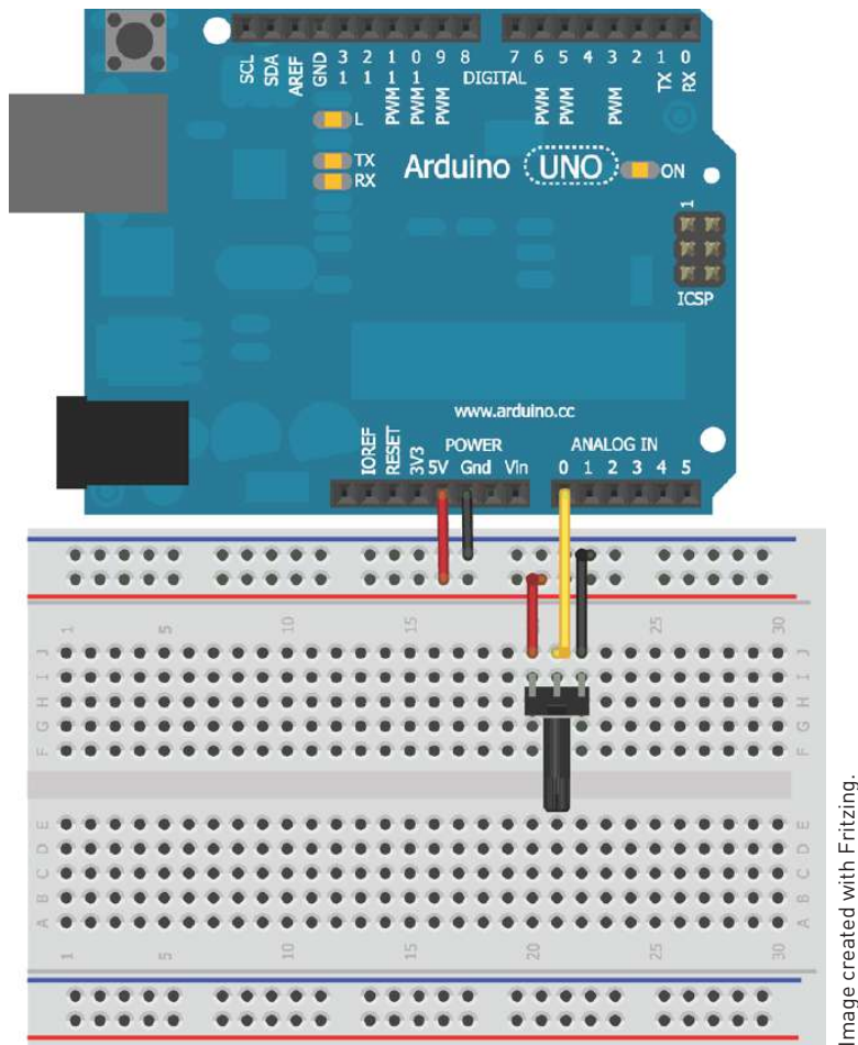
Figure 3-3: Potentiometer circuit
