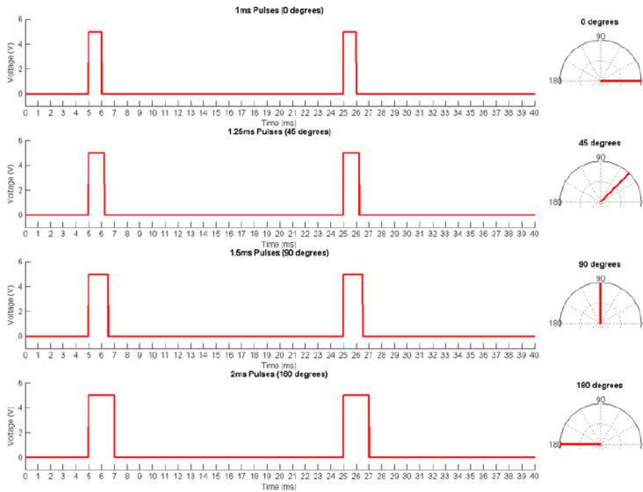
Figure 4-10: Servo motor timing diagram
